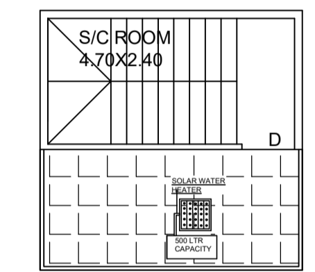
PROPOSED TERRACE FLOOR PLAN
